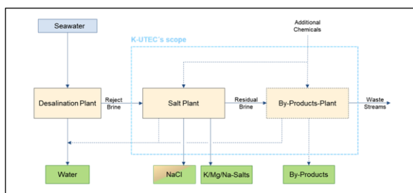
Fig. 2: General flow chart of the project (K-UTEK). N.b. although the project's scope is focused on salt recovery and by-products, the necessary analysis and linkages with the green hydrogen industry and desalination plants will be established, such as heat integration analysis and benefits for green hydrogen production costs.
